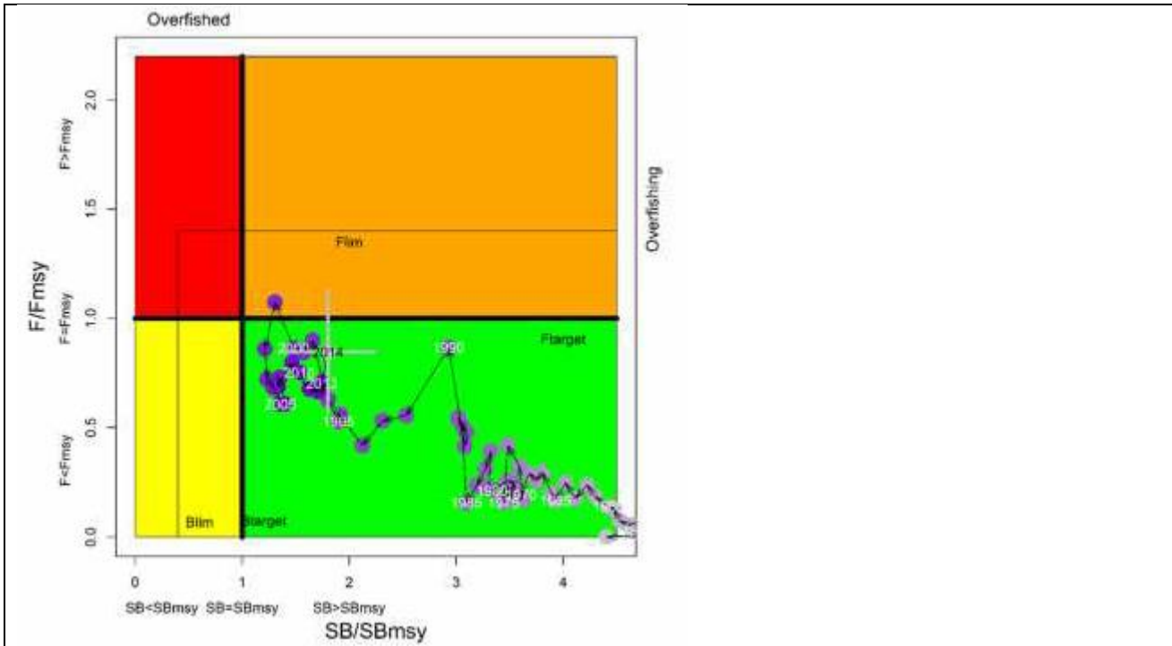
Figure 1. Albacore: SS3 Aggregated Indian Ocean assessment Kobe plot. Blue circles indicate the trajectory of the point estimates for the SB ratio and F ratio for each year 1950–2014 (the grey lines represent the 80 percentiles of the 2014 estimate). Target ( F_{target} and SB_{target} ) and limit ( F_{lim} and SB_{lim} ) reference points are shown.
