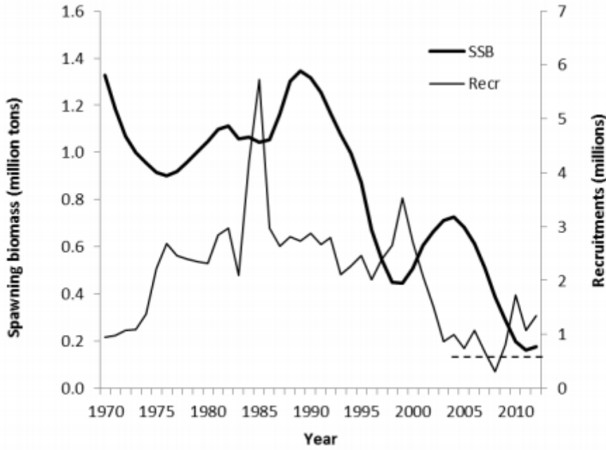
Spawning biomass (SSB) and recruitment (Recr) of jack mackerel. From the October 2013 stock assessment (R5).
