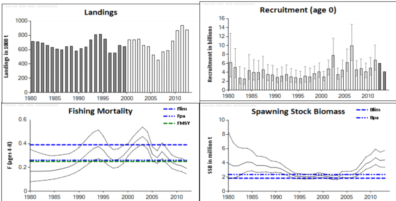
Mackerel in the Northeast Atlantic. From the ICES advice, May 2014.
