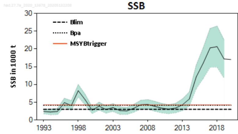
Figure 2. Haddock in Division 7a. Summary of the stock assessment with the state of the stock relative to the biomass reference points.
