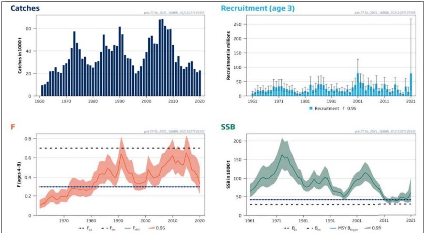
FIGURE 1. SAITHE IN DIVISION 5.B (FAROES GROUNDS). SUMMARY OF THE STOCK ASSESSMENT. CATCHES, RECRUITMENT, FISHING MORTALITY (F), AND SPAWNING-STOCK BIOMASS (SSB) (ICES, 2021).
