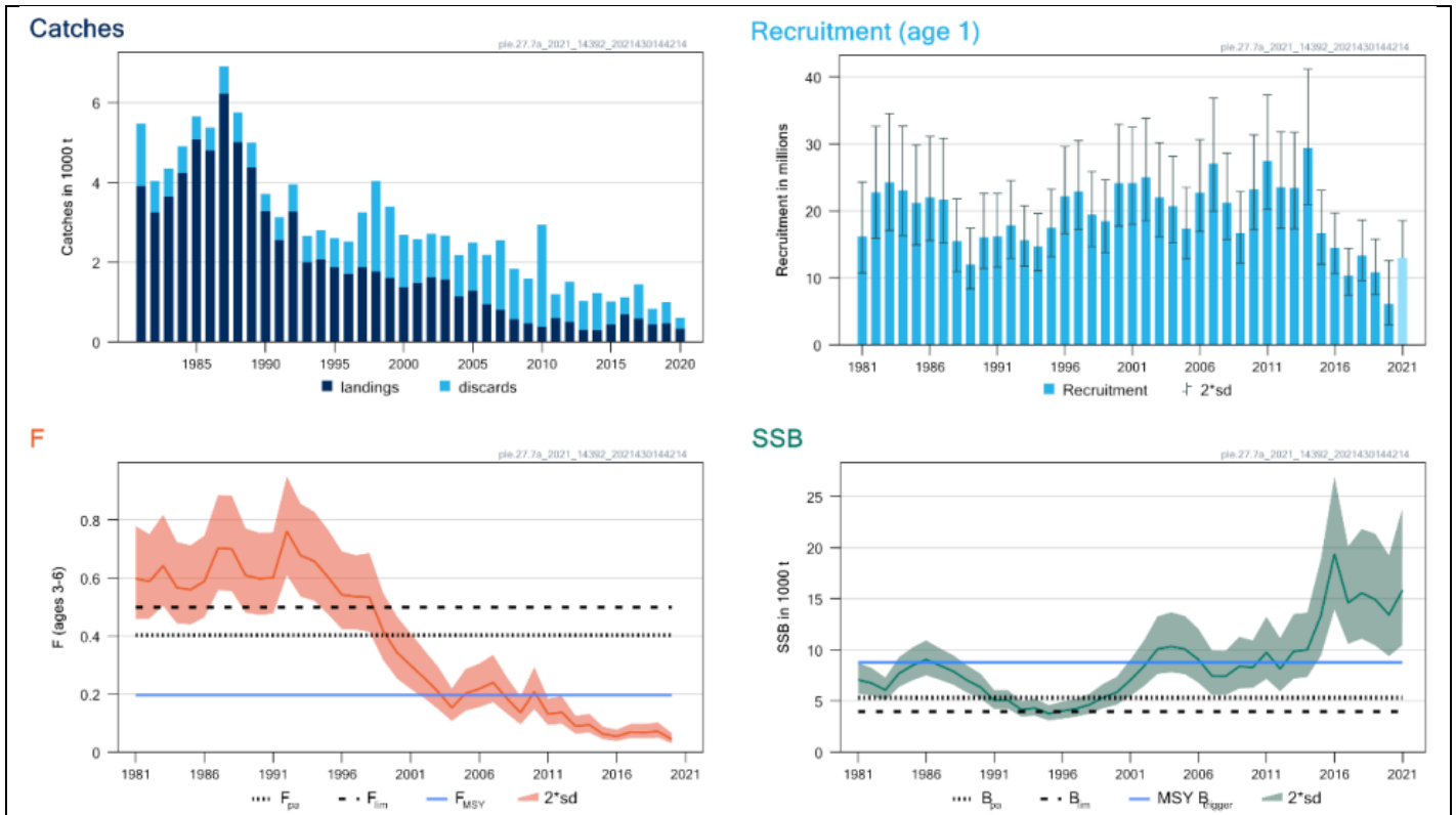
FIGURE 1. PLAICE IN DIVISION 7.A. SUMMARY OF THE STOCK ASSESSMENT. THE ASSUMED RECRUITMENT VALUE FOR 2021 IS SHADED IN A LIGHTER COLOUR (SOURCE: ICES. 2021)
