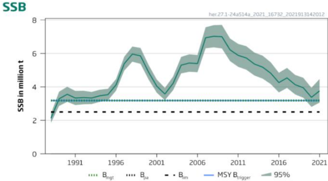
FIGURE 2. HERRING IN SUBAREAS 1,2,5 AND DIVISIONS 4.A AND 14.A. BIOMASS RELATIVE TO B_{MSY} .
