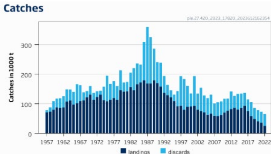
Figure 1. Long-term catch (including discards) trends for plaice in subarea 4 and subdivision 3.a.20 from 1957 to 2022 (ICES, 2023).
