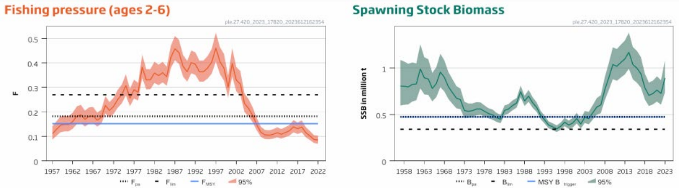
Figure 2. Plaice in subarea 4 and Subdivision 3.a.20 (North Sea and Skagerrak) summary of the stock assessment.
