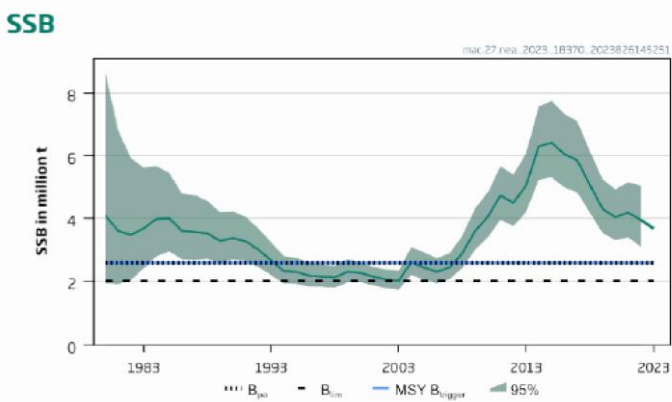
Figure 2. Spawning-stock size above MSY B_{trigger} , B_{pa} , and B_{lim} for Mackerel in subareas 1–8 and 14, and in Division 9.a (ICES 2023)
