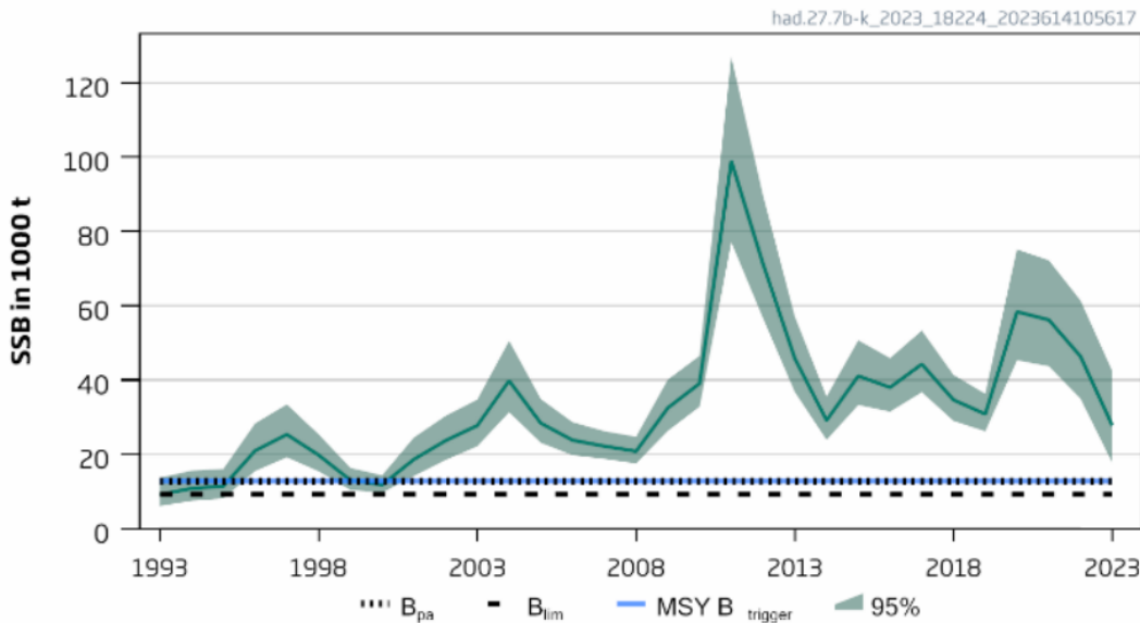
Figure 2. ICES spawning stock biomass for haddock in Divisions 7.b-k (ICES 2023).
