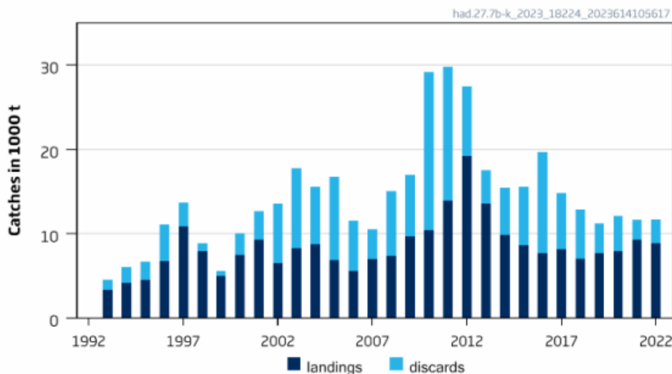
Figure 1. Haddock catches in Divisions 7.b-k (ICES 2023).
