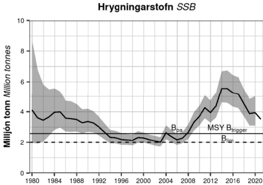
Figure 2. Mackerel in ICES Division 5.a. Spawning stock biomass.
