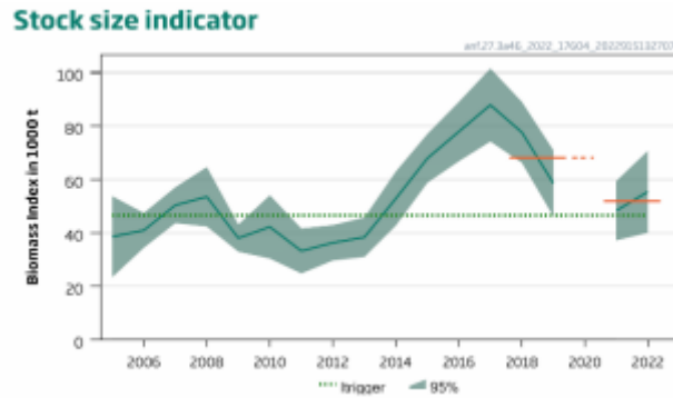
Figure 2. Anglerfish in subareas 4 and 6, and in Division 3.a. Stock biomass from the SIAMISS-Q2 survey. The horizontal orange lines indicate the average of the most recent two years, and the previous three years (with 2020 not available and therefore excluded from the average). Source: ICES, 2022.
