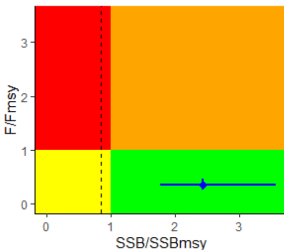
Figure 1. Latest estimate of SSB_{\text{recent (2015 - 2018)}/SSB_{\text{MSY}}} and F_{\text{recent (201 - 2017)}/F_{\text{MSY}}} for WCPO yellowfin (blue dot, with range (80% CIs) indicated by bars). Dashed black line = limit reference point.
